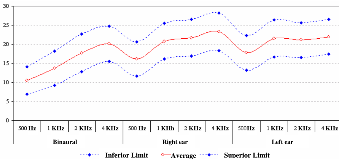
Figure 1. Interval of confidence to the gap limiar in miliseconds obtained by RGDT test in the binaural and monoaural to the right and left ear presentation in the group of preschool born term.
