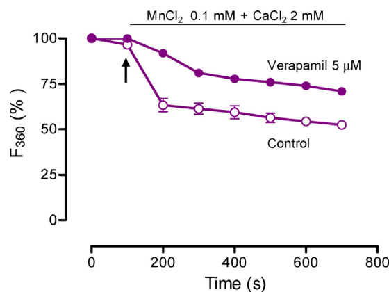
Fig. 6. Quenching of fura-2 fluorescence, induced by \text{Mn}^{2+} , obtained in the absence and presence of verapamil (5 \mu\text{M} ). Fura-2-loaded cardiomyocytes after 6 days in culture were incubated with verapamil (5 \mu\text{M} ), for 10 min. The arrow indicates the incubation of \text{MnCl}_2 . The symbols and vertical bars are means \pm SEM ( n=3 ).
