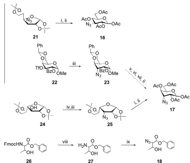
Scheme 1. Synthesis of the azido-functionalized sugars 3- N_3 -Glc 16 and 3- N_3 -Gul 17 , and the amino acid N_3 -ThrOBn 18 . Reagents and conditions: (i) TFA 80%, rt; (ii) Ac_2O , Py, rt; (iii) NaN_3 , 120–130 °C; (iv) Tf_2O , DCM–Py (19:1); (v) NaOMe, MeOH; (vi) AcOH 80%, microwave heating (110 °C, 15 min); (vii) Ph_3CBF_4 , DCM, rt; (viii) 20% piperidine/DMF, rt; (ix) Tf_2O , NaN_3 ; CuSO_4 , H_2O , MeOH, CH_2Cl_2 , rt.
